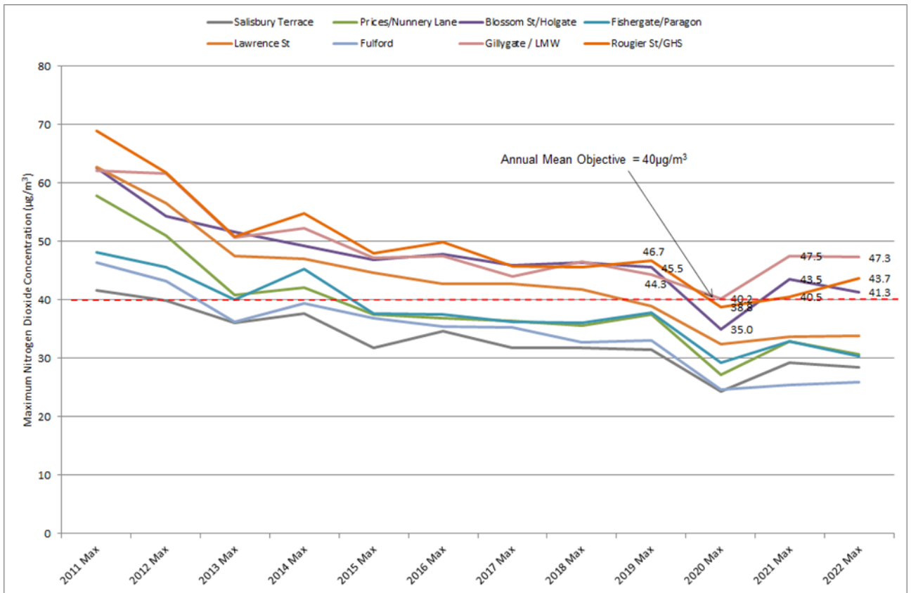
Figure 2. 2 Maximum NO 2 concentrations monitored at a relevant location across key areas of the current AQMA
