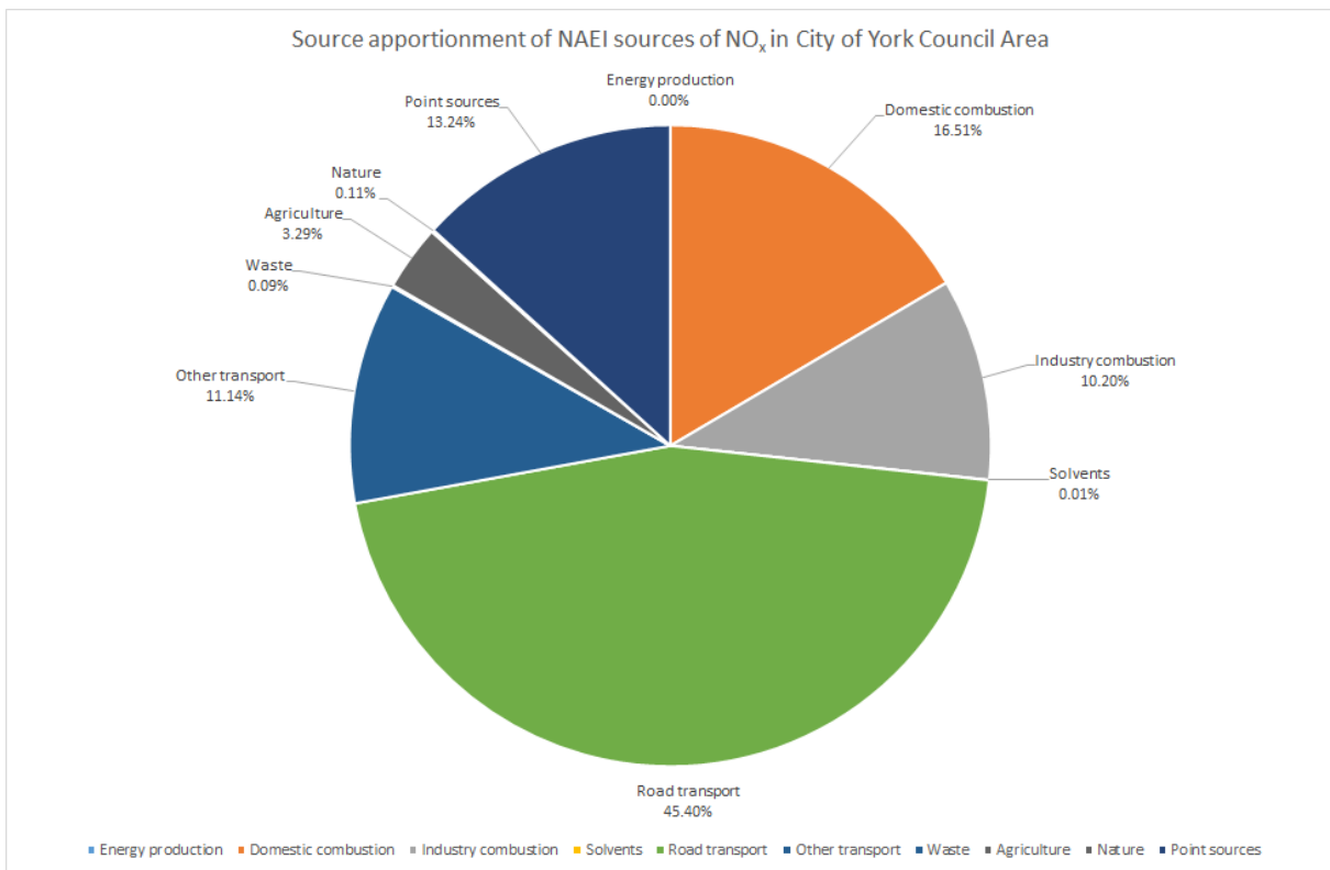
Figure 3.3 Source apportionment of NAEI sources of NO x in CYC's area
